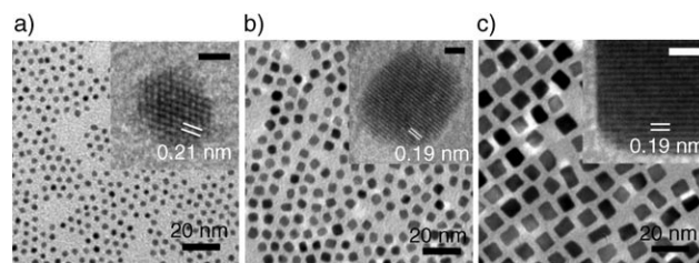
Figure 1. Representative TEM images of a) the 3 nm polyhedral b) the 5 nm truncated cubic and c) the 7 nm cubic Pt NPs. The insets are the representative HRTEM images of corresponding single particles, showing a) Pt(111), b) Pt(100), and c) Pt(100) lattice fringes. All scale bars in the insets correspond to 1 nm.
