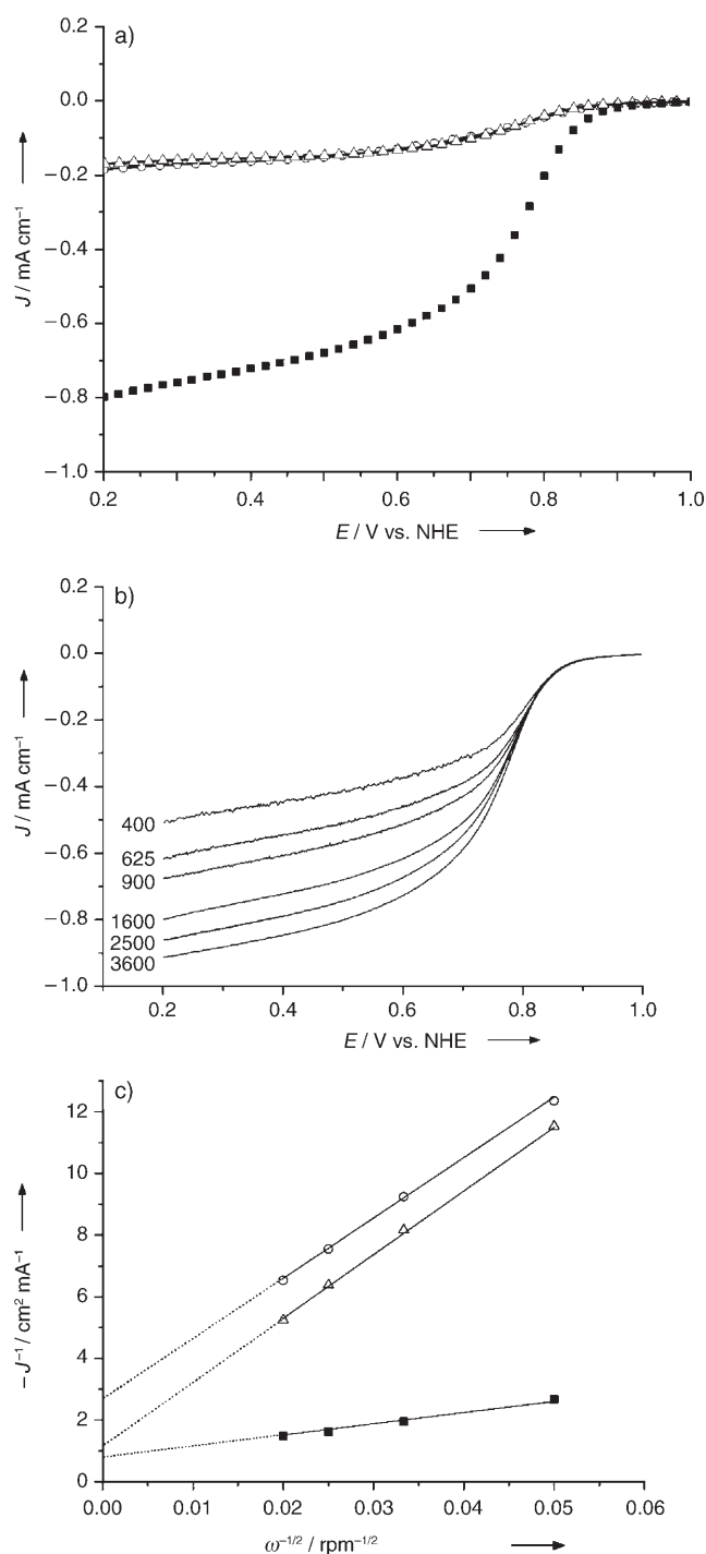
Figure 4. a) Disk current densities in oxygen saturated 0.5 M \text{H}_2\text{SO}_4 as a function of potential the platinum catalysts ( \circ polyhedron, \Delta truncated cube, \blacksquare cube) at a rotation speed of 1600 rpm. b) Rotation-rate-dependent current-potential curves for 7 nm platinum nanocubes. c) Koutecky-Levich plots at 0.6 V for the platinum catalysts ( \Delta polyhedron, \circ truncated cube, \blacksquare cube). The potential was applied with scanning rate of 10 \text{ mVs}^{-1} .
